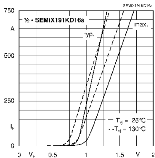
Fig. 7: On-state characteristics
